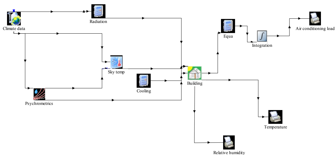
Figure 4. Assembly of modules for building description in TRNSYS.
